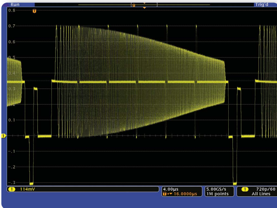
► Figure 14b. Effects of a roll off above 20 MHz.
