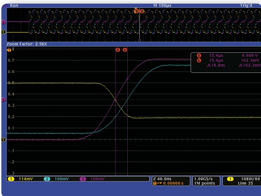
▶ Figure 13b. Measuring the delay in the Pb signal due to an additional length of cable or processing time.
