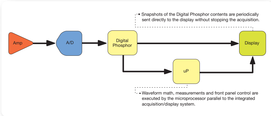
► Figure 5. Parallel-processing architecture of a digital phosphor oscilloscope (DPO).
