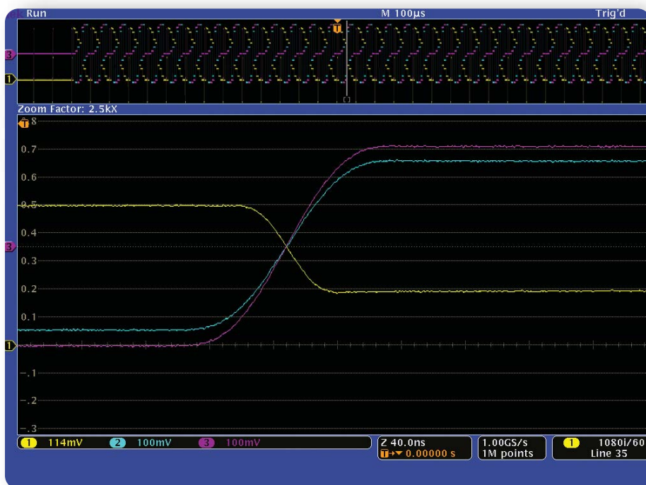
▶ Figure 13a. Correct timing of the luminance (Y) and the color-difference signals (Pb and Pr) during the green to magenta transition of a 100% color bar signal.
