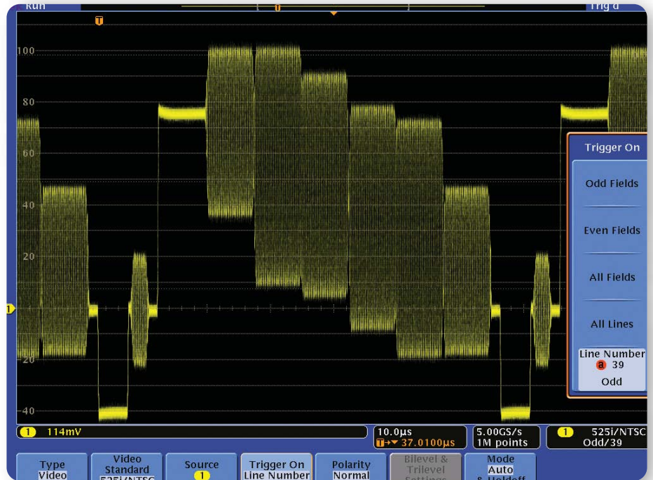
► Figure 6. The 4000 Series' video trigger allows convenient selection of video standard, source, component to trigger on, polarity, and holdoff settings. In this example, the oscilloscope has triggered on line 39 of the Odd Field of an NTSC signal.
