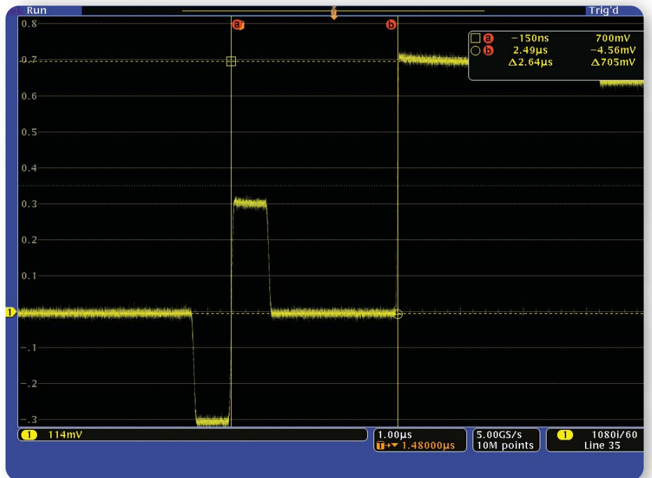
▶ Figure 11. Using cursors to measure the Y signal white level amplitude and the time from O_H to the start of active video in a 1080i/60 HDTV 100% color bar signal.
