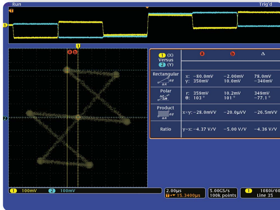
▶ Figure 15. The 4000 Series' XY mode used to view a vectorscope-like display. Screen cursors with polar readouts indicate the magnitude and phase of the red vector.
