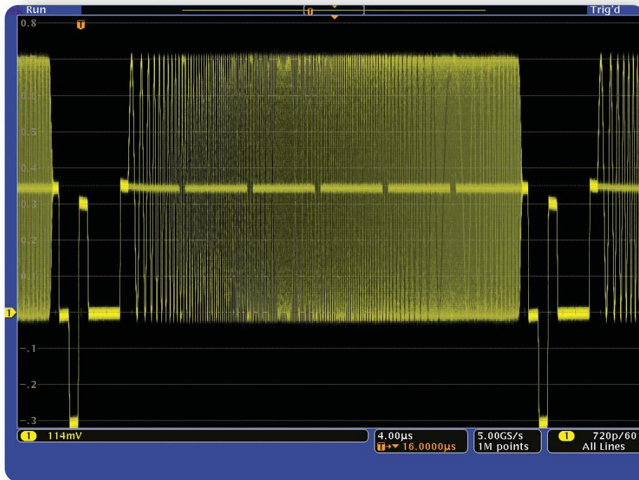
► Figure 14a. Line sweep of an analog HDTV signal with no frequency roll off—a pure signal.
