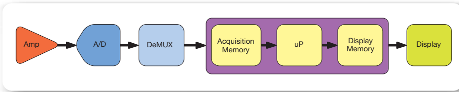
► Figure 4. Serial-processing architecture of a digital storage oscilloscope (DSO).
